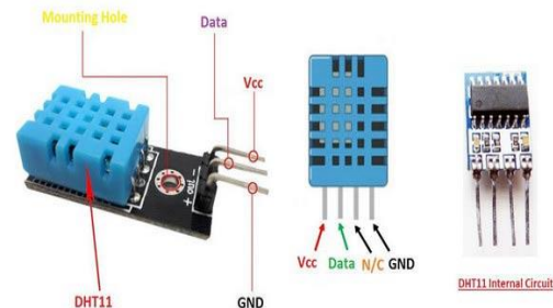
Gambar 2. Sensor DHT-11
