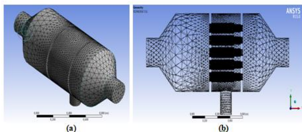
Gambar 2. Meshing model deliquidiser (a) isometric view (b) front view
