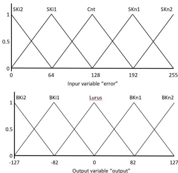
Gambar 9. Fuzzy set input dan output Fuzzy Logic Controller
