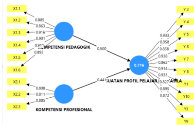
Gambar 2 Model Struktural SEM-PLS
