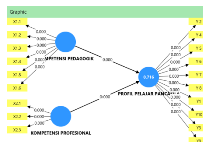
Gambar 3 Model Hasil Bootstrapping
