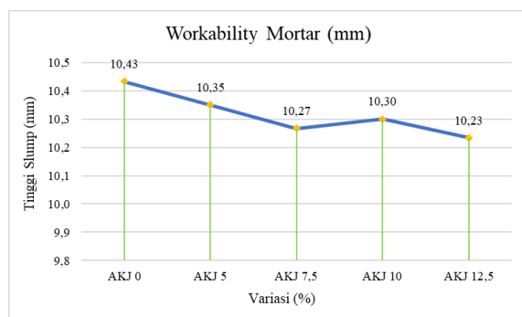
Gambar 3. Grafik Workability Mortar
