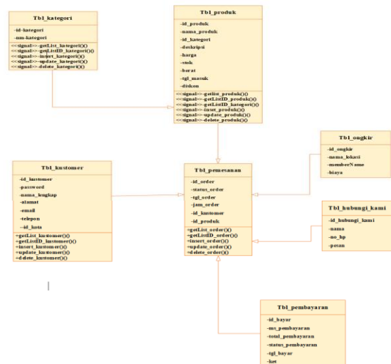
Gambar 2 : Class Diagram
