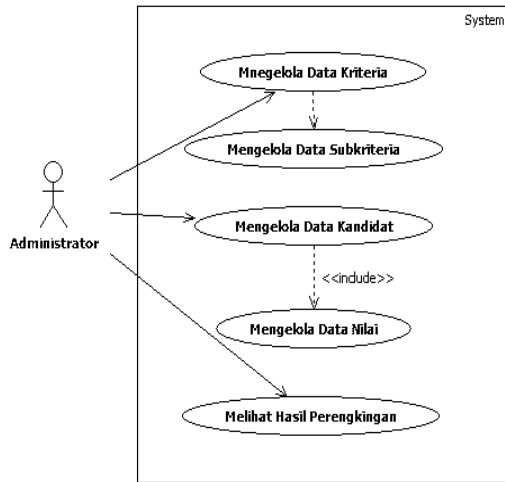
Gambar 1: Use Case
