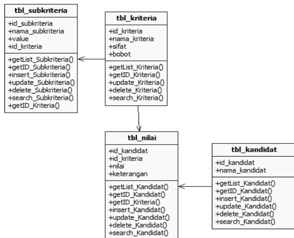
Gambar 7 : Class Diagram
