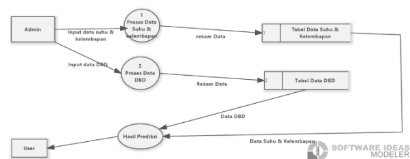
Gambar 2 DFD Level 1
