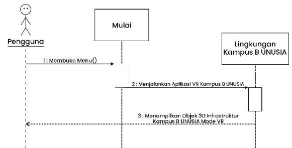
Gambar 7 Sequence Diagram Menu Mulai
