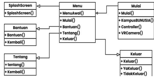
Gambar 12 Class Diagram
