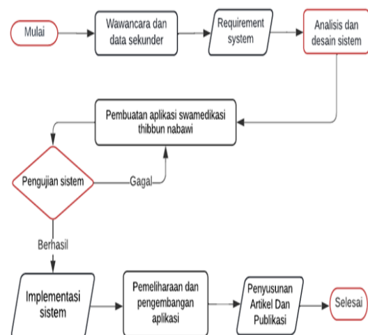
Gambar 1. Alur penelitian
