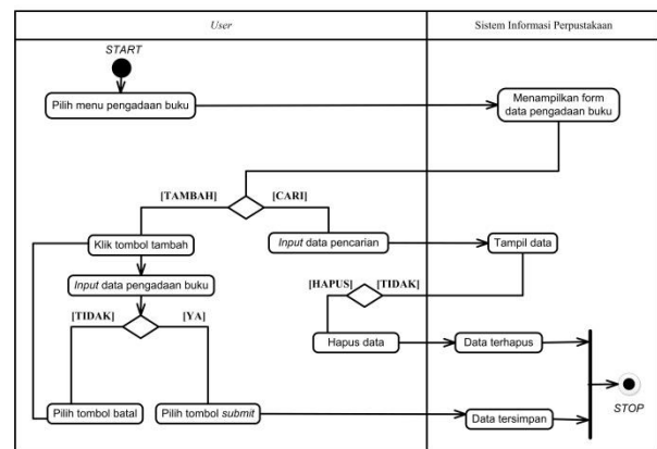
Gambar 4 Activity Diagram Pengadaan Buku
